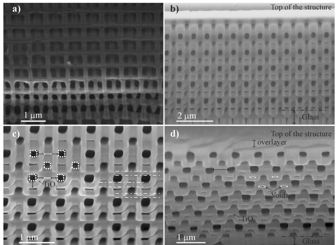
Figure 1. SEM images of (a) polymer, (b,c) partially \text{TiO}_2 infiltrated woodpile structures, and (d) nearly completely infiltrated structures obtained after 1500 and 4500 ALD cycles, respectively. The polymer template has been removed by calcination (b–d). Cross-sections are cut using a focus ion beam with viewing angles (a) 40^\circ (b,c) 45^\circ and (d) 25^\circ . In the enlarged image (c) of the partially \text{TiO}_2 infiltrated woodpile shown in (b), the dotted circles and dashed lines represent the rod positions in the initial polymer template; the \text{TiO}_2 is indicated by black lines while the interspaces between two \text{TiO}_2 hollow channels are highlighted by the full white lines. The image in (d) reveals the presence of residual air voids (dotted circles) inside the inverted titanium dioxide structure. The metal oxide over-layer on the top of the structure is also shown.
