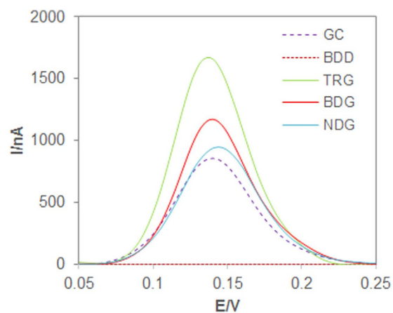
Figure 3. DPV profiles for the determination of catechin at concentrations of 12.0 \mu\text{M} on glassy carbon (GC), boron doped diamond (BDD), thermally reduced graphene (TRG), boron doped graphene (BDG) and nitrogen doped graphene (NDG) electrodes. Conditions: 100 mM phosphate buffer, pH 7.3; step potential 4 mV, modulation amplitude 25 mV.
