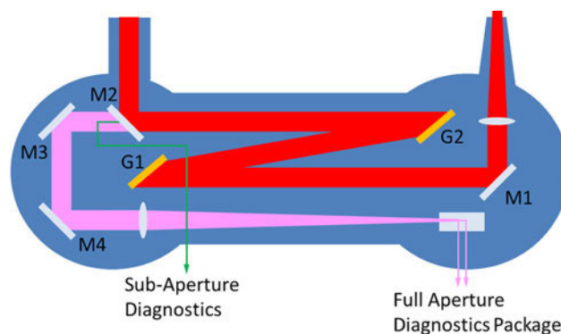
Figure 10. Schematic of the Vulcan short pulse diagnostics in TAP. The main pulse follows the red path, the full aperture beam the pink path and the sub-aperture diagnostics the green path.
