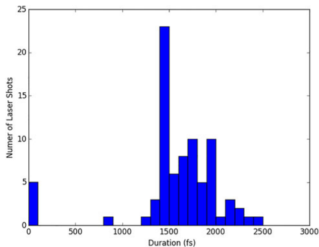
Figure 20. Histogram of pulse durations recorded during an experimental campaign in TAW.
