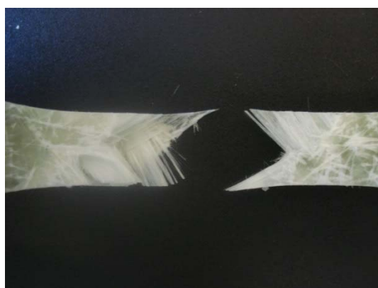
b) Failure of off-axis tests samples , 45^\circ
