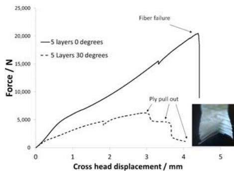
Typical Force Vs cross head displacement curves for tests samples of 5 layers. 3,1 \times 10^{-4} \text{ s}^{-1} .
