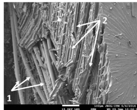
Typical failure test sample for 45°. V_f = 36,5, 3,1 \times 10^{-4} \text{ s}^{-1} .
