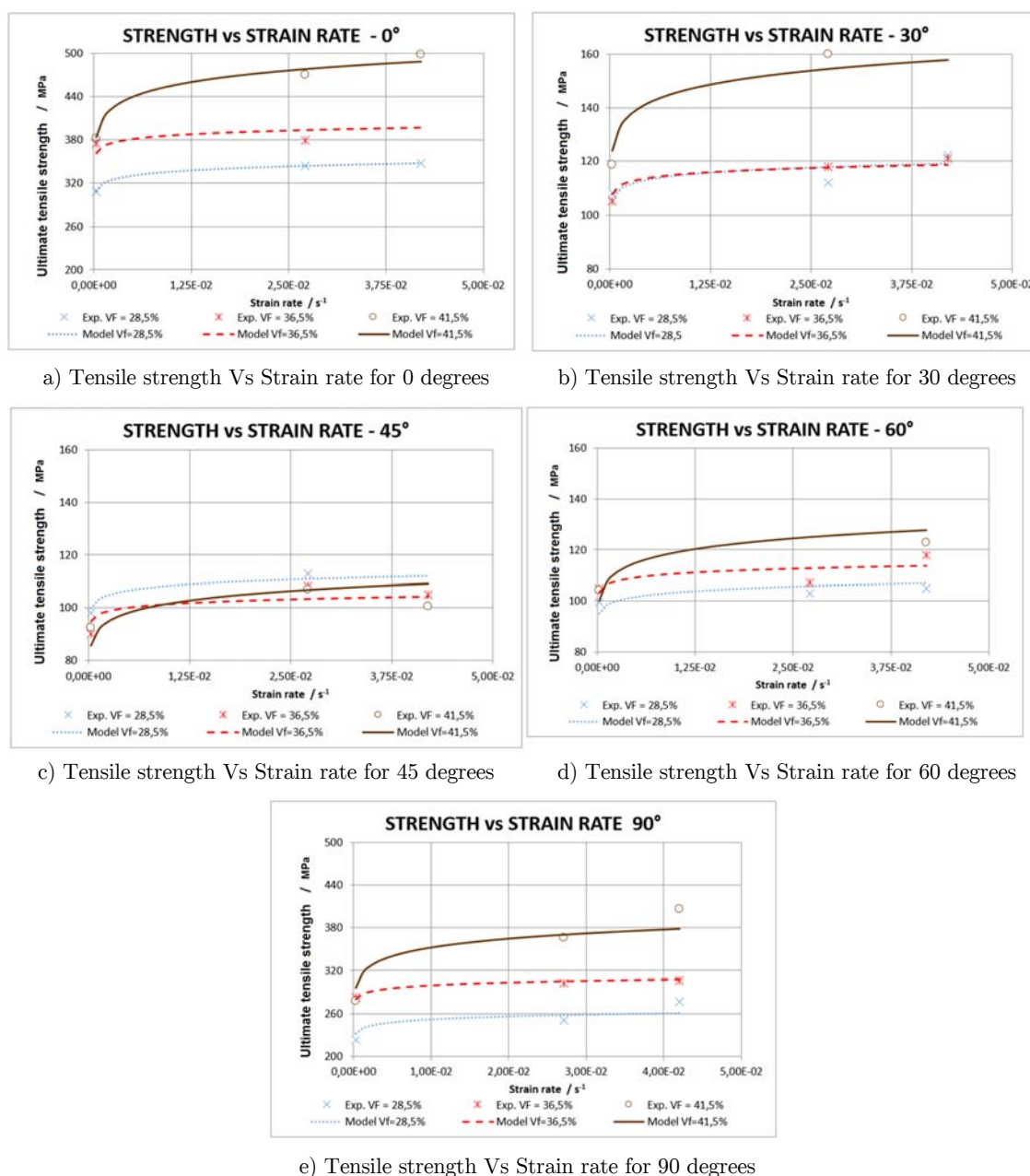
Figure 4: Tensile strength Vs strain rate. Model and experimental results.
