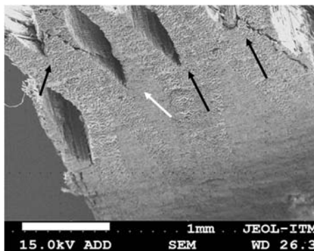
e) Detail of Figure d. Black arrows show cracks growing through the plies. White arrow shows cracks growing through the matrix
