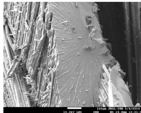
f) Failure in the matrix. Test sample at 45°. V_f = 36,5, 3,1 \times 10^{-4} \text{ s}^{-1}
