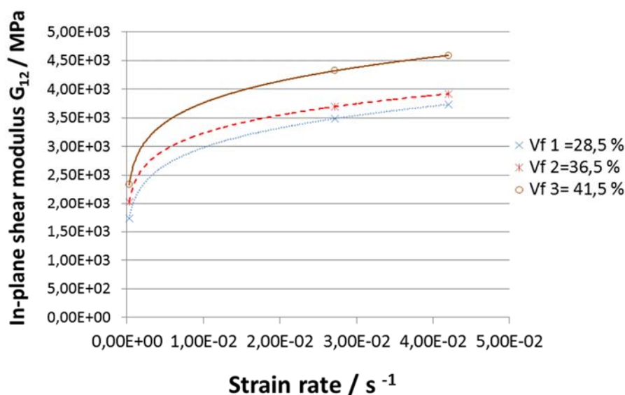
Figure 9: In-plane shear modulus G_{12} vs strain rate.
