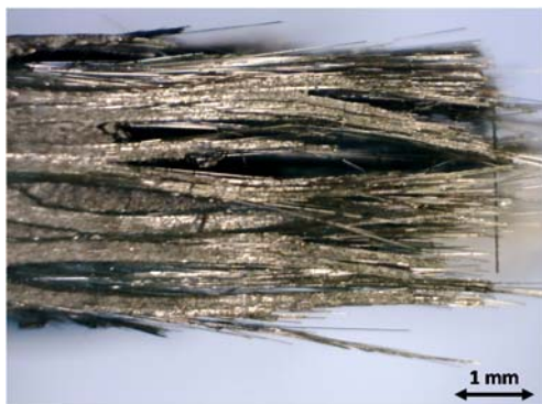
Test sample for 0°, V_f = 36,5, 3,1 \times 10^{-4} \text{ s}^{-1} .
