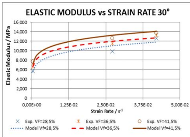
b) Elastic Modulus Vs Strain rate for 30 degrees
