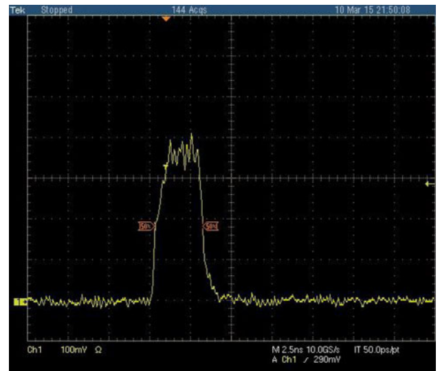
Figure 4. Temporal profile of the ASE beam.
