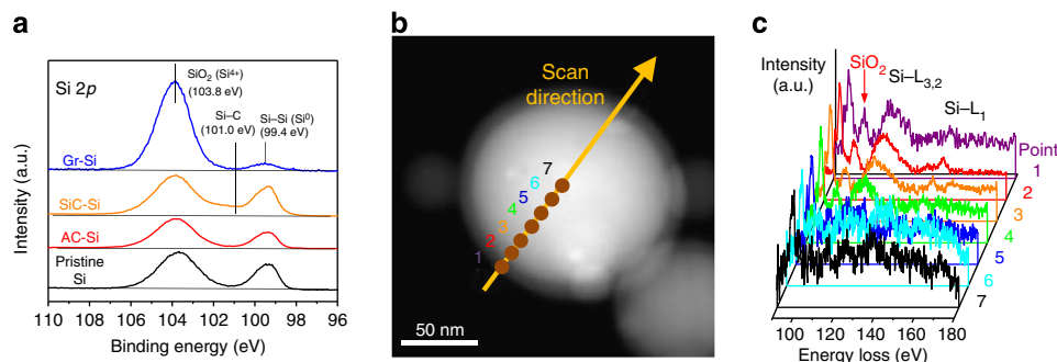
Figure 2 | Verification of SiC-free growth. (a) X-ray photoelectron spectroscopy spectra in Si 2p band for Gr-Si, SiC-Si, AC-Si and pristine Si. (b) A scanning TEM image of a Gr-Si NP. (c) EELS spectra for the spots denoted in b.
